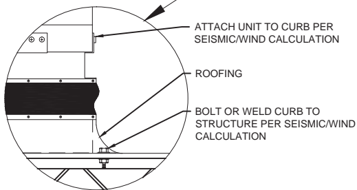
STEEL ATTACHMENT
