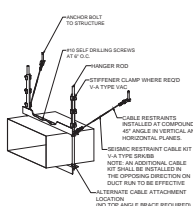
Detail 3 - Combination Cable Restraint (Option #1)
