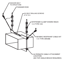
Detail 1 - Transverse Cable Restraint (Option #1)
