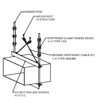
Detail 2 - Transverse Cable Restraint (Option #2)
