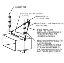
Detail 4 - Combination Cable Restraint (Option #2)
