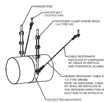
Detail 5 - Combination Cable Restraint (Round)
